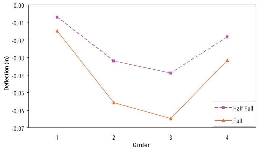
c. Deflection Profile
