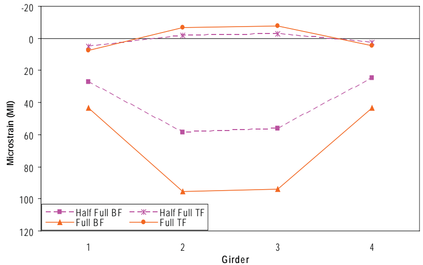
b. Strain Profile
