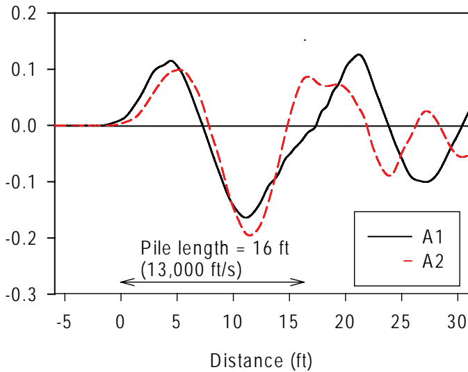
Pile integrity test results, with pile toe estimated to be 16 feet below ground level (measured wave speed = 13,000 feet/second)
