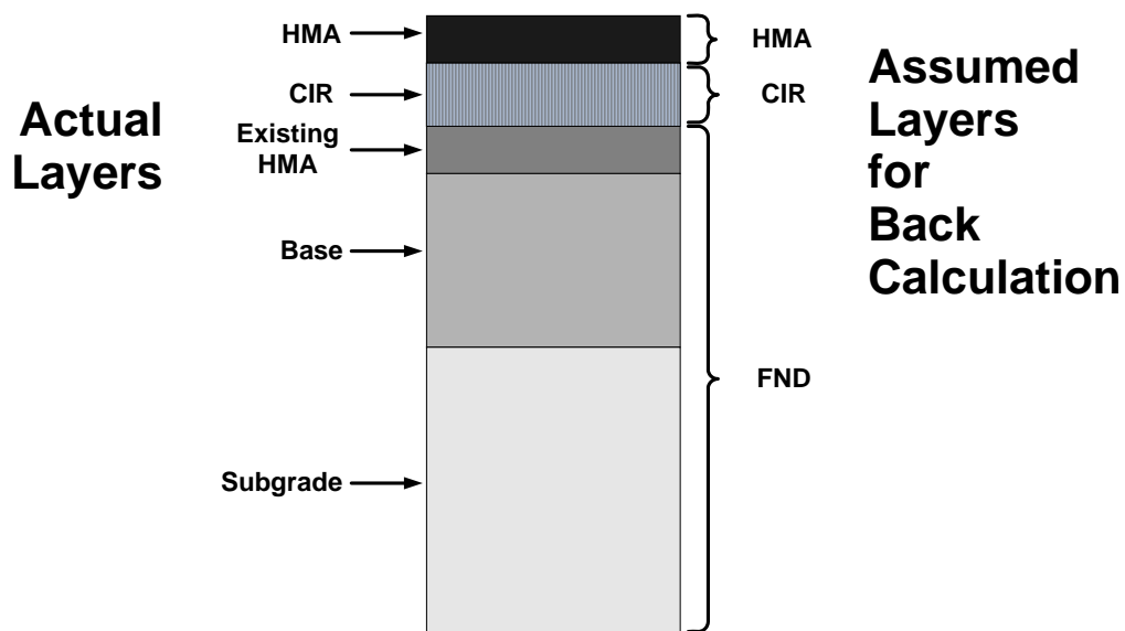
Figure 5. Pavement layers for back calculation purposes
