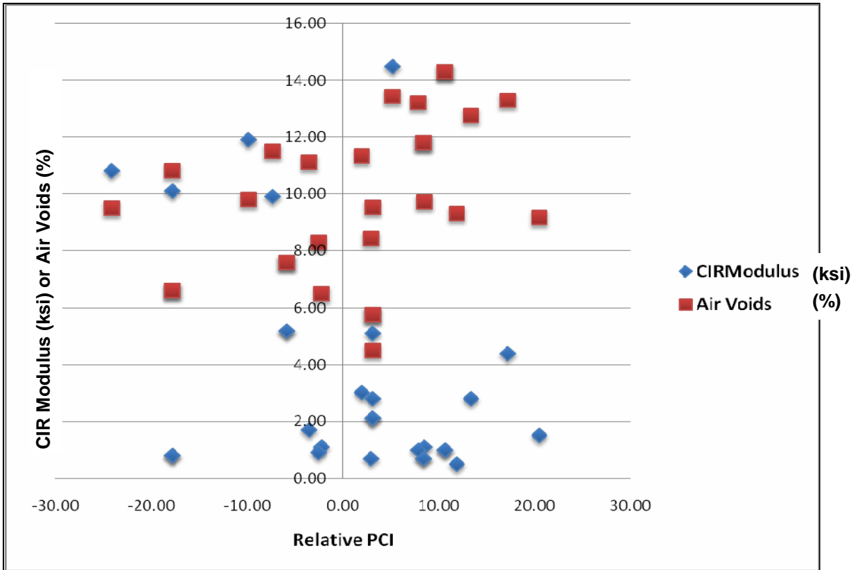
Figure 15. Selected material properties vs. relative PCI
