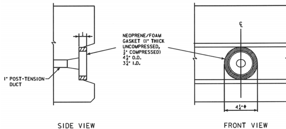
Figure 14. Post-tensioning tendon gasket detail (dimensions in inches).
