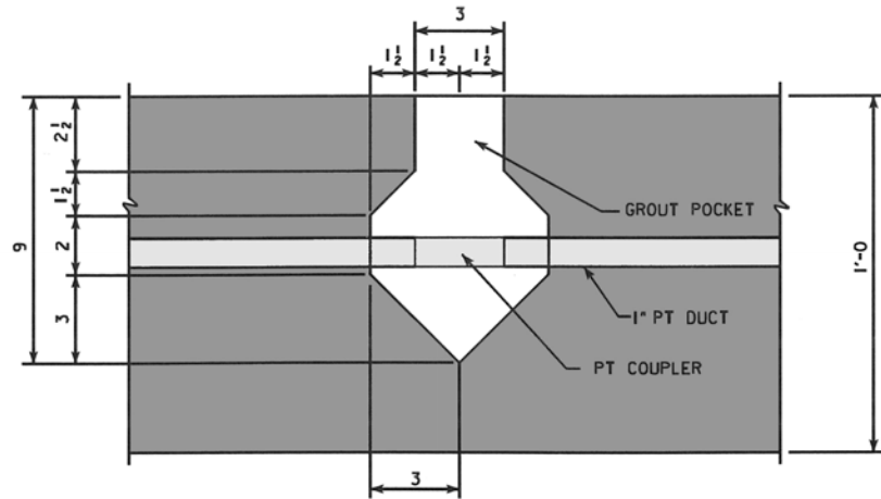
Figure 13. Keyway dimensions for the longitudinal joint (dimensions in inches).
