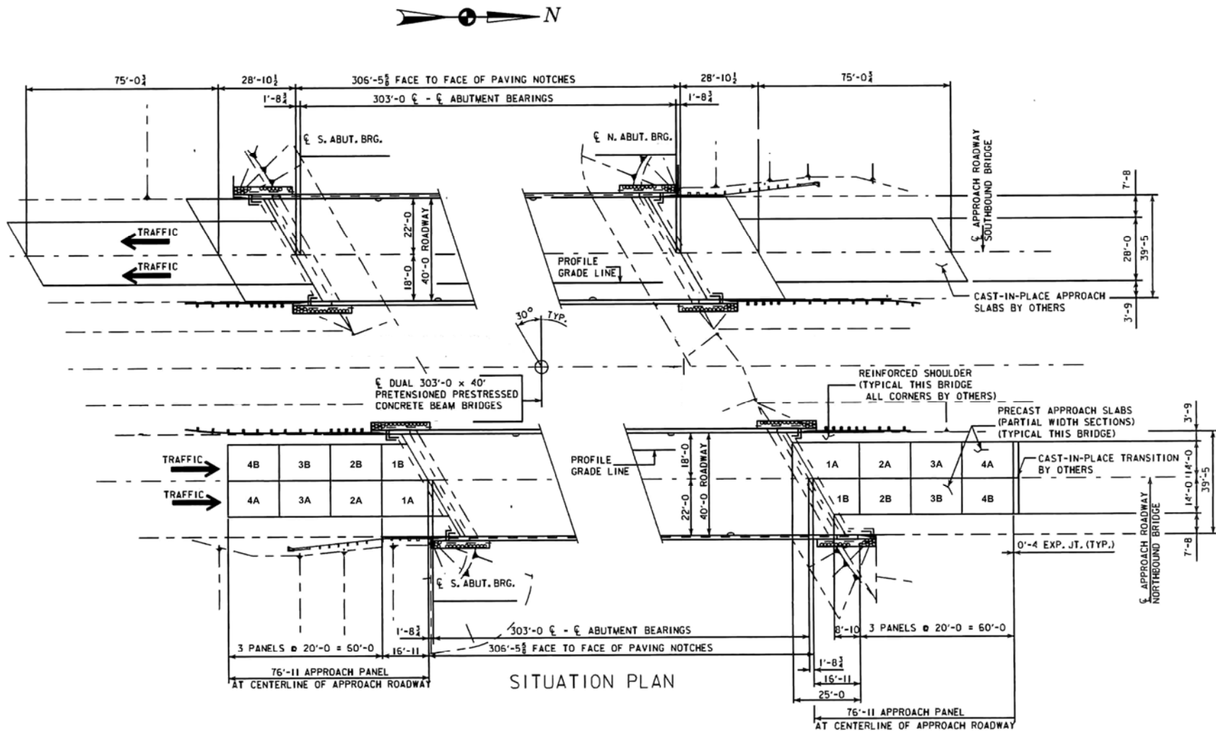
Figure 3. Situation Plan for the Highway 60 bridge and precast approach slabs.
