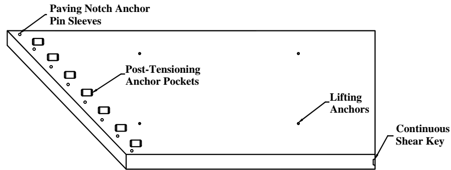
Figure 9. Approach slab Abutment Panels.
