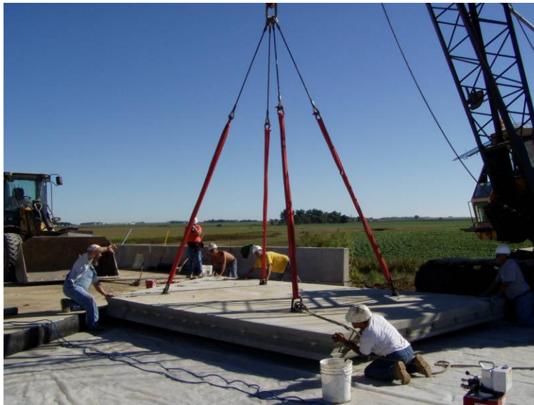
Figure 25. Installation of Panel 1A at the south bridge abutment.
