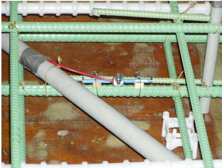
Figure 40. Vibrating wire strain gage mounted in the precast panel during fabrication.
