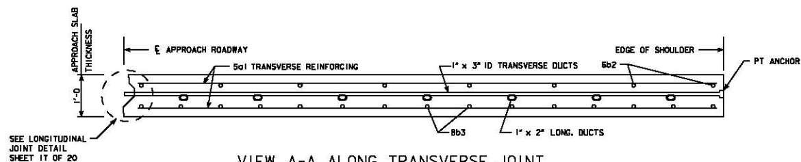
VIEW A-A ALONG TRANSVERSE JOINT
