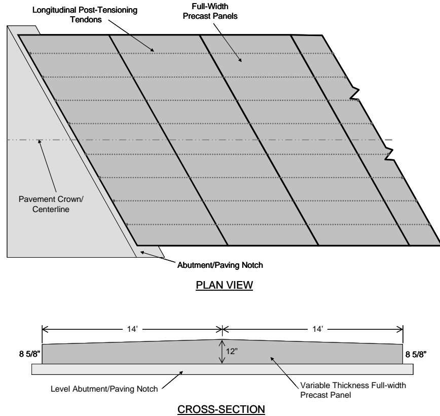
Figure 4. Schematic layout of full-width panels with variable thickness.
