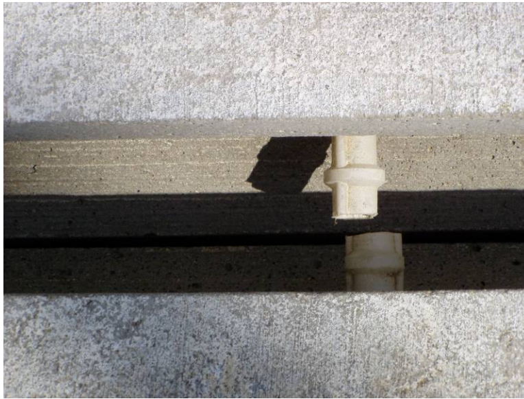
Figure 39. Slight misalignment of transverse post-tensioning ducts at the longitudinal joint.
