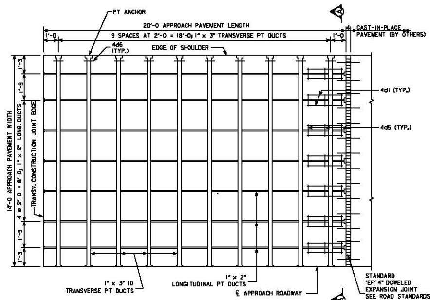
PLAN VIEW SHOWING POST-TENSIONING DUCTS TRANSVERSELY AND LONGITUDINALLY
