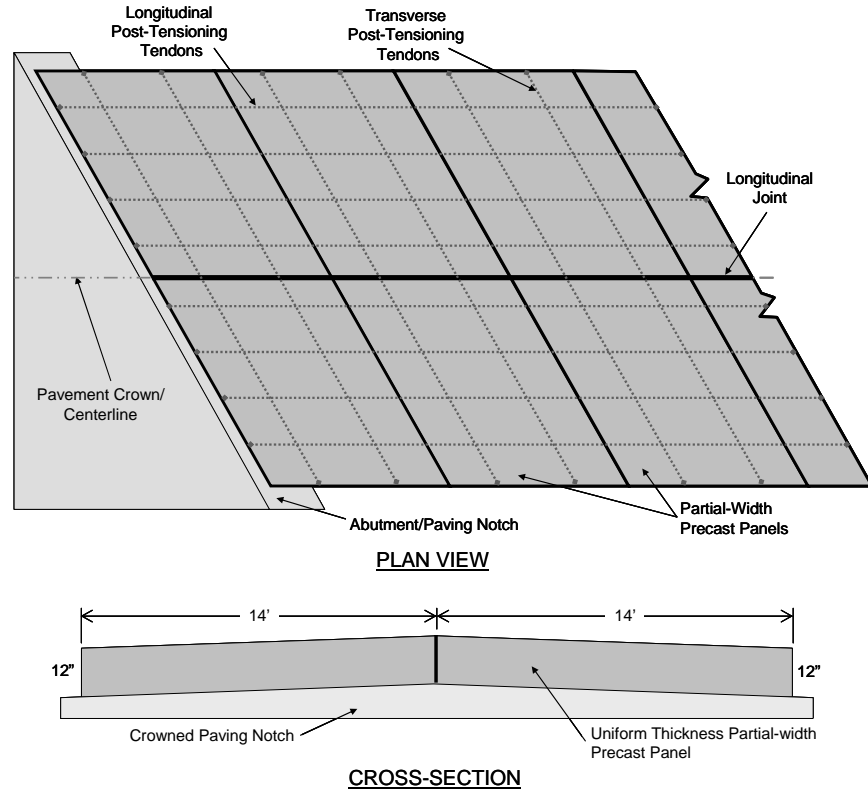
Figure 5. Schematic layout of partial width panels with uniform thickness.
