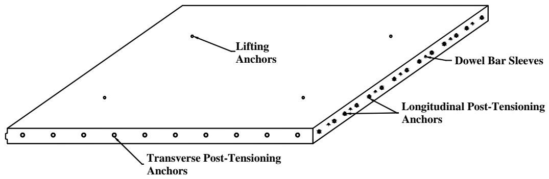
Figure 11. Approach slab Joint Panels.
