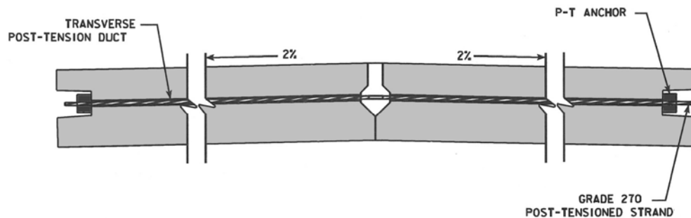
Figure 8. Longitudinal joint at the centerline of the approach slab.
