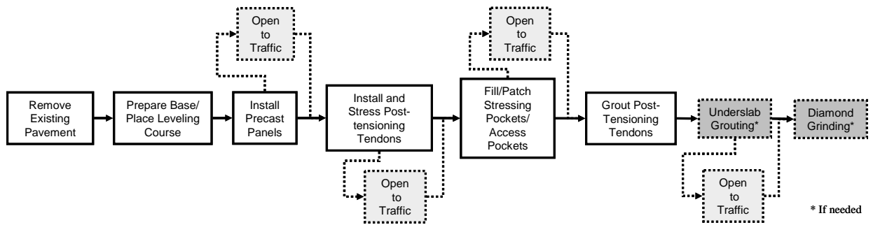
Figure 1. Flowchart for the overall PPCP construction process.
