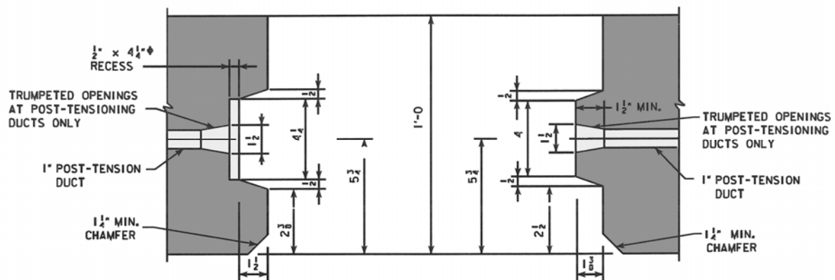
Figure 12. Transverse keyway dimensions for the precast panels (dimensions in inches).
