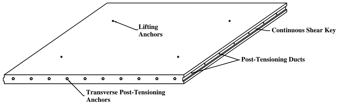
Figure 10. Approach slab Base Panels.
