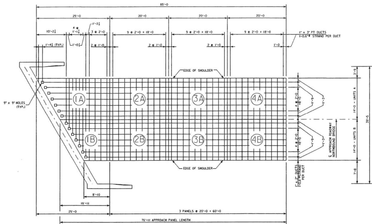
Figure 6. Selected precast panel and post-tensioning tendon layout.
