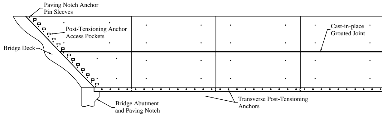
Figure 7. Selected precast panel layout.
