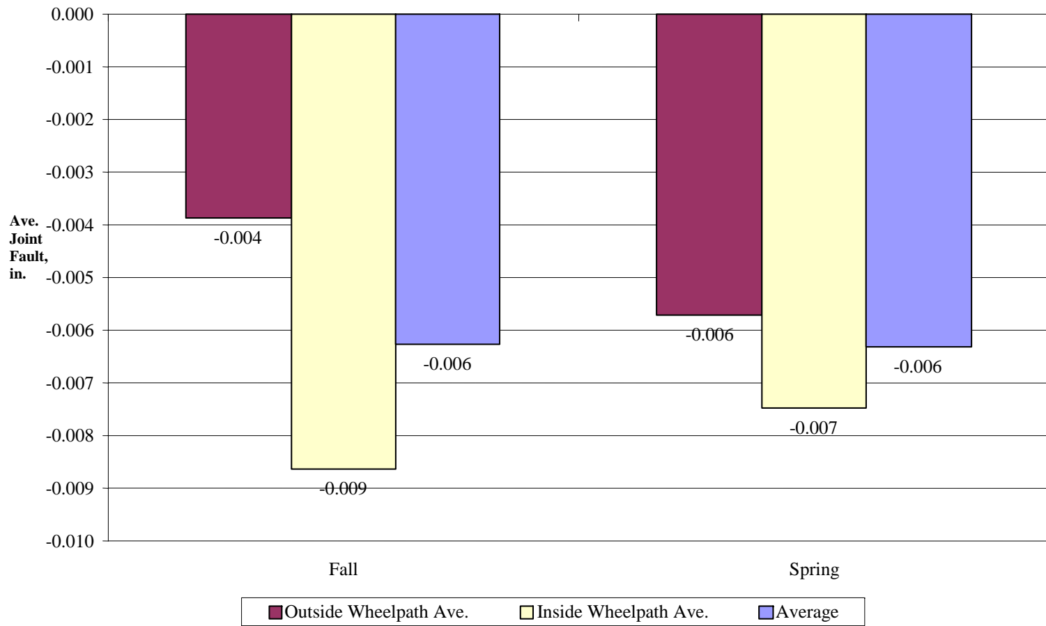
Figure C.7. Seasonal Effect on Faulting
