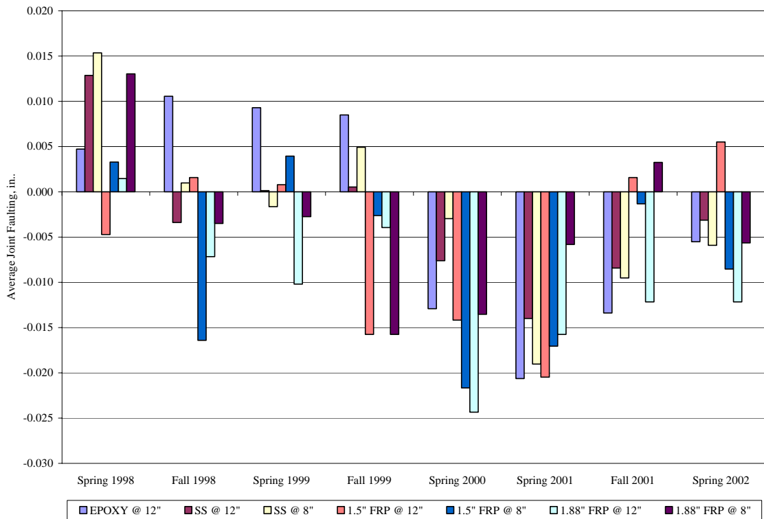
Figure C.4. Average Faulting ~ Outside Wheel Path
