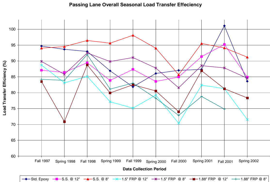
Figure C.2. Passing Lane Overall Seasonal Load Transfer Efficiency
