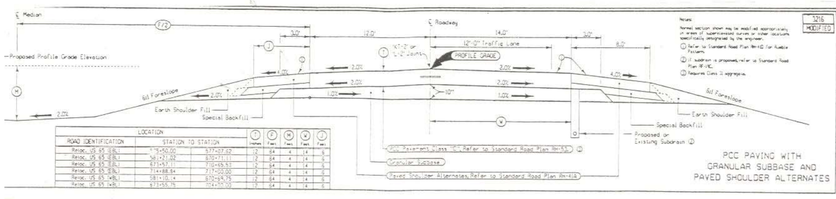
Figure A.1. Typical Project Cross Section
