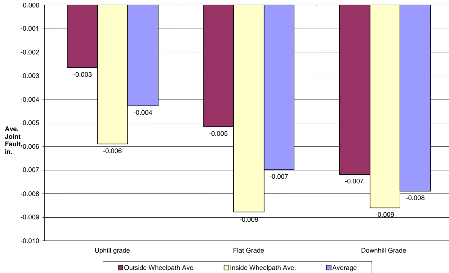
Figure C.6. Grade Effect on Faulting
