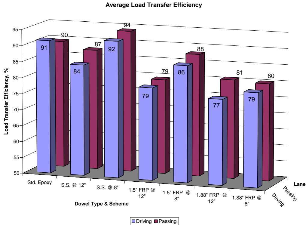
Figure 7. Average Load Transfer Efficiency
