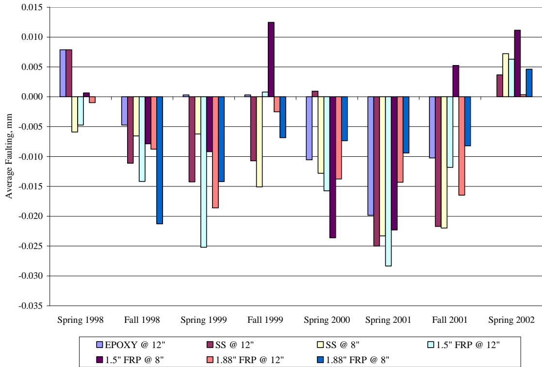
Figure C.3. Average Faulting ~ Inside Wheel Path
