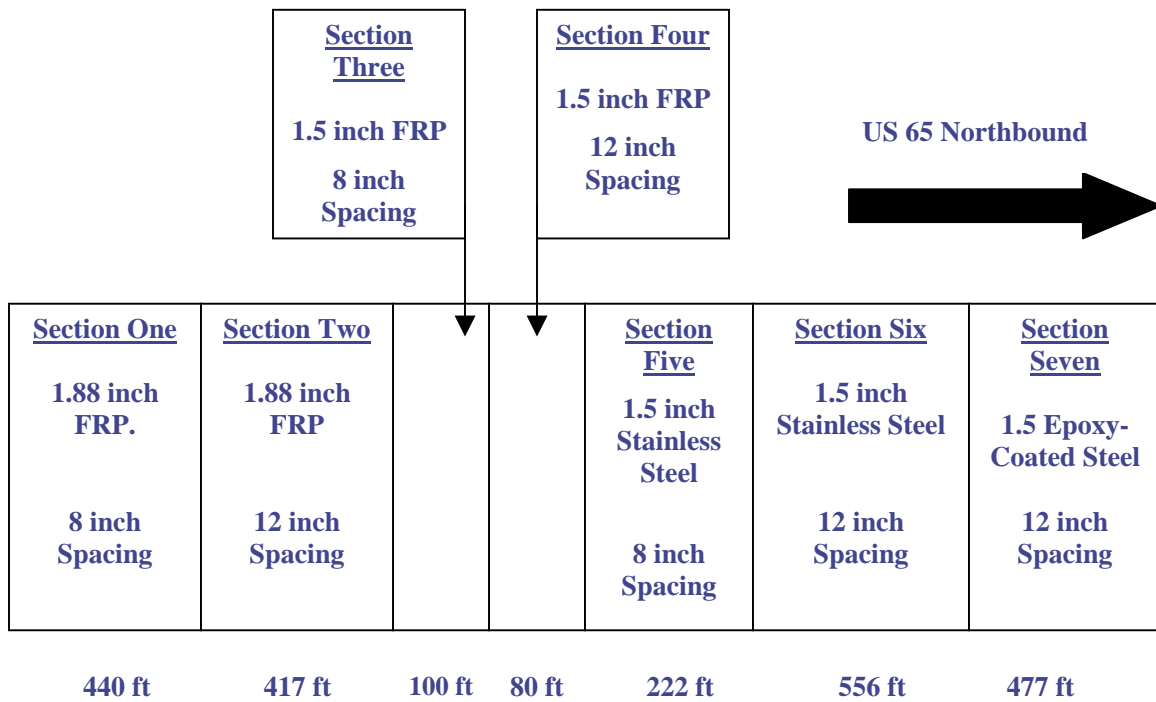
Figure 2. Site Layout of Test Sections
