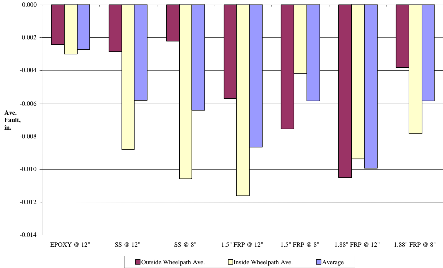
Figure C.5. Average Faulting Over Research Period
