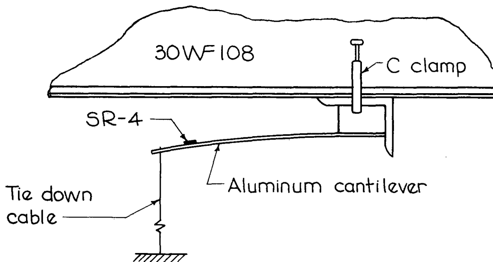
DEFLECTION GAGE
