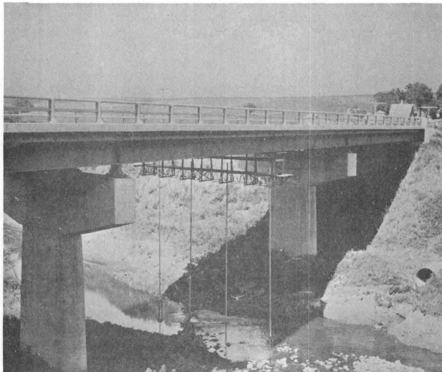
Photo 2: Bridge, showing falsework erected for installing deflection gages.
