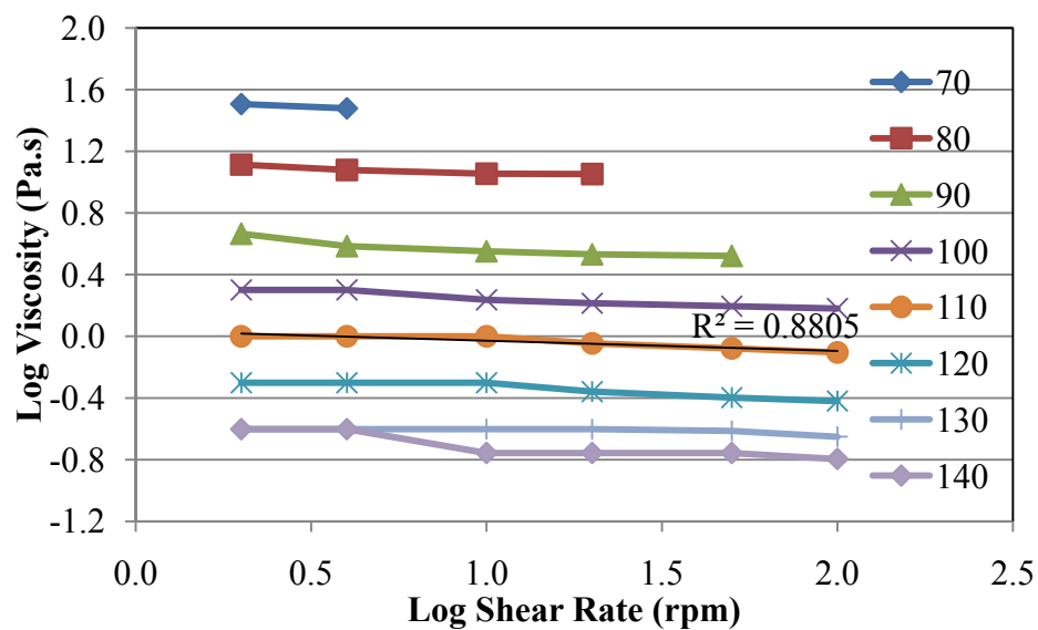
Figure C7.38. Power-law Relationship for Blend 20
