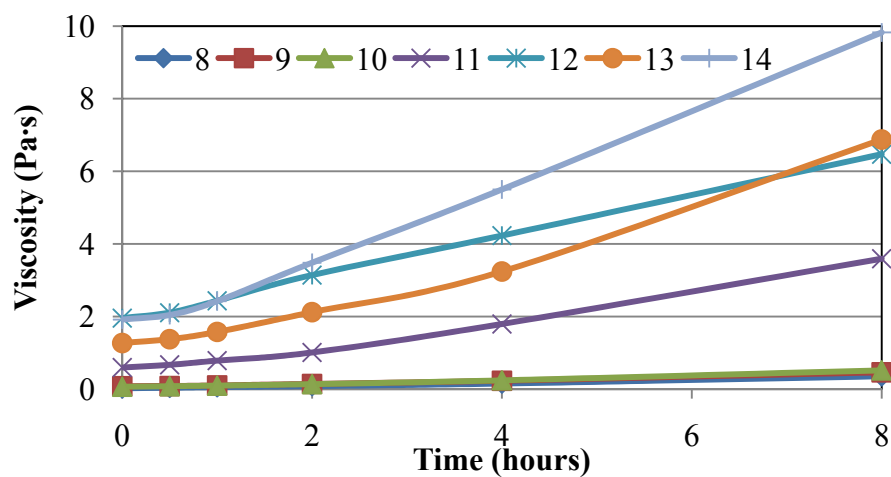
Figure 4.2. Viscosity over Time for Switchgrass Blends before Treatment at 125°C
