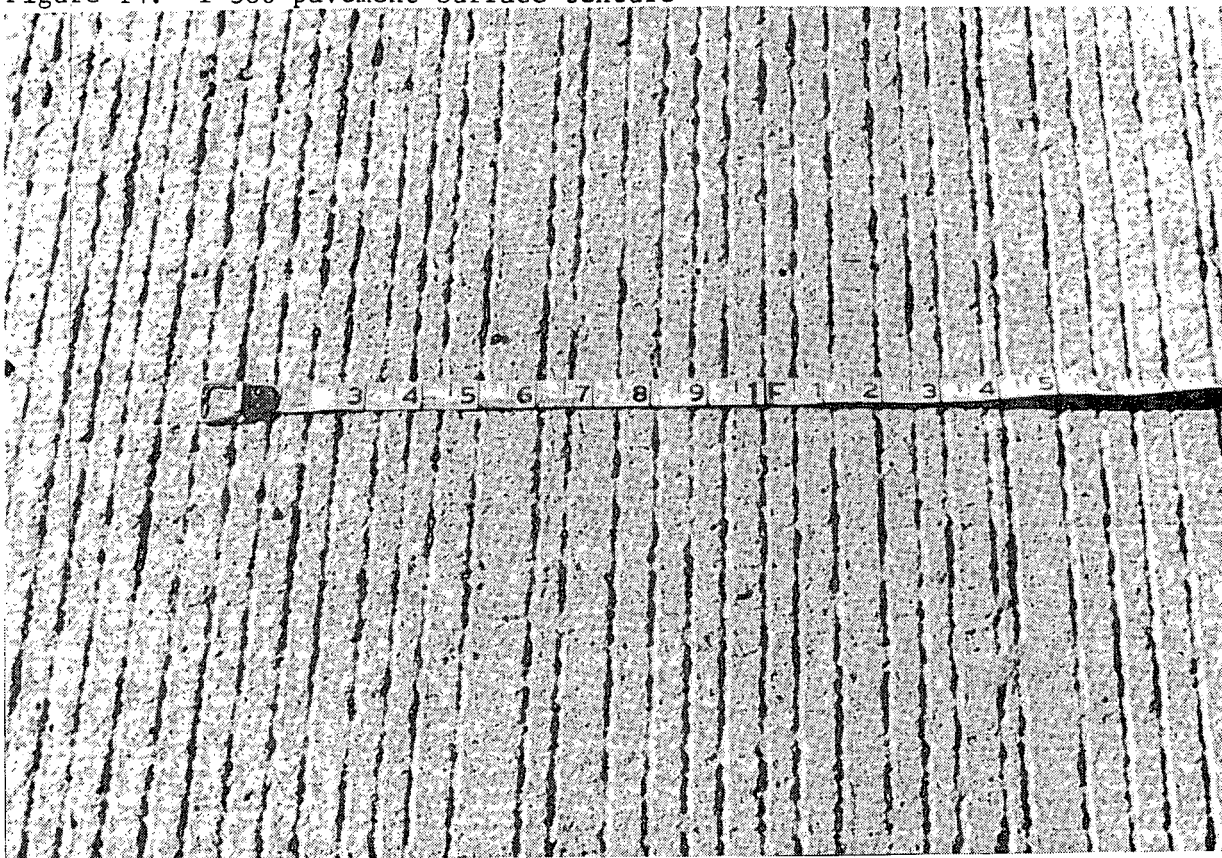
Figure 14. I-380 pavement surface texture
