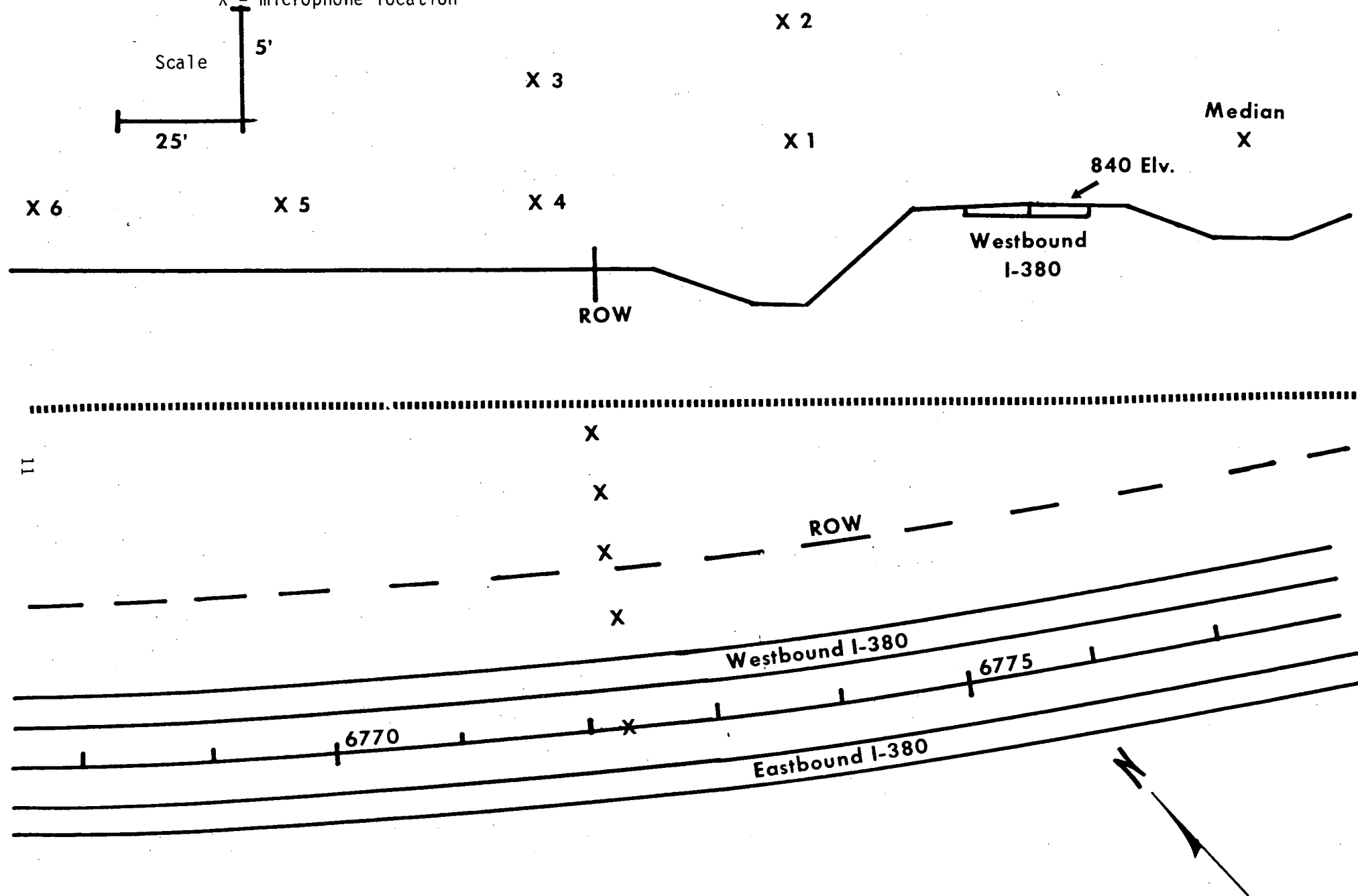
Figure 6. Cross section and plan view of free field site X = microphone location
