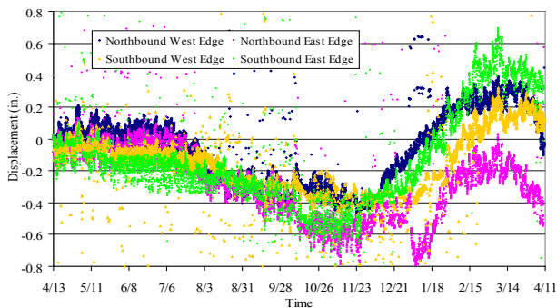
Figure 2. Longitudinal abutment displacements (south end) for both bridges
