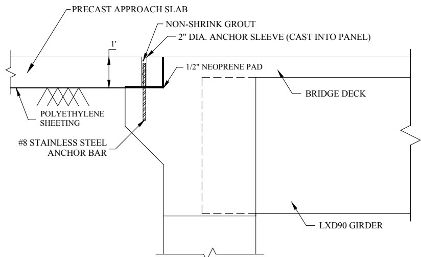
Figure 1. Connection detail for the precast approach slab to abutment, northbound
