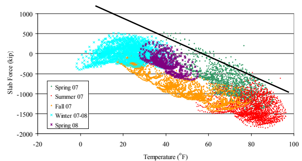
Figure 3. Northbound bridge approach slab average force with respect to slab temperature
