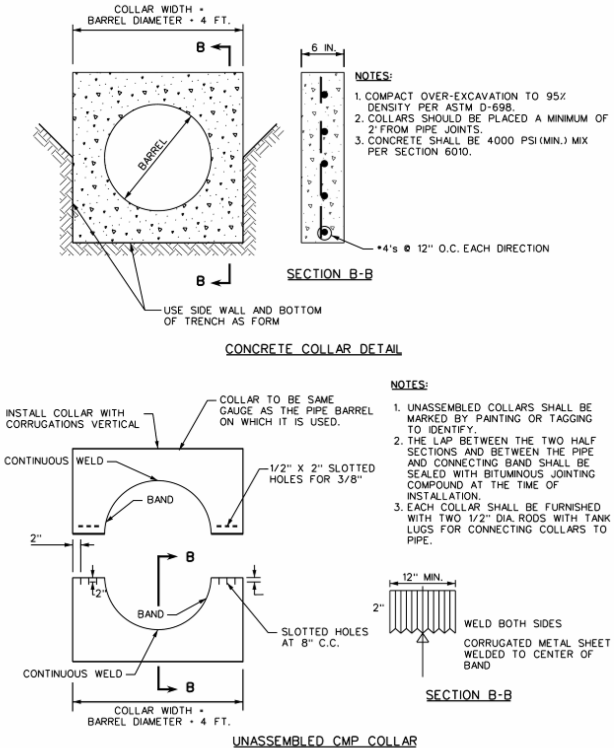
Figure 8: Anti-seep collars
