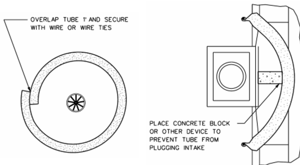
Figure 1: Filter tubes used for inlet protection
