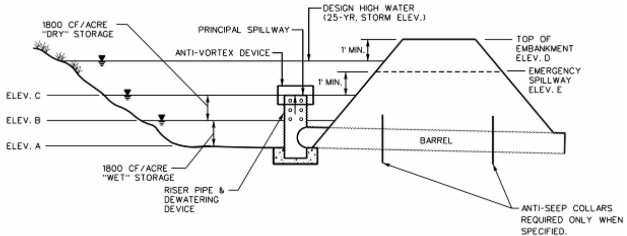
Sediment basin with emergency spillway
