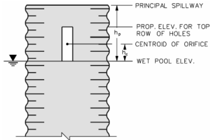
Figure 5: Theoretical discharge orifice for design of perforated risers
