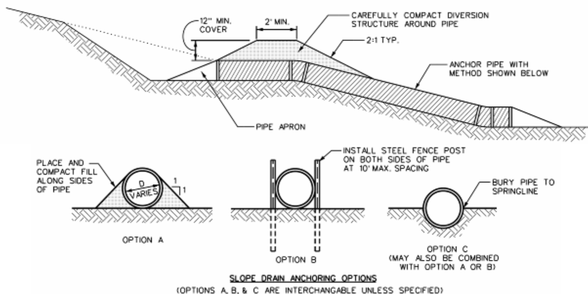
Figure 1: Temporary slope drain
