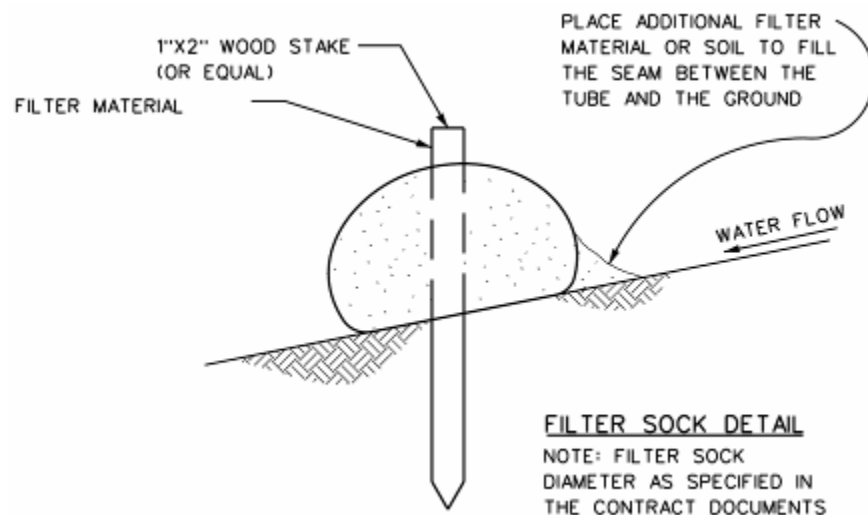
Figure 1: Typical filter sock installation
