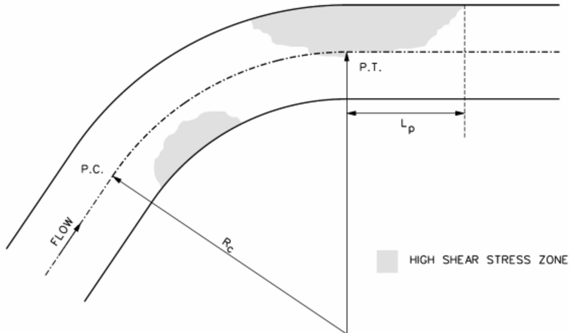
Figure 3: Shear stress distribution in a channel bend
