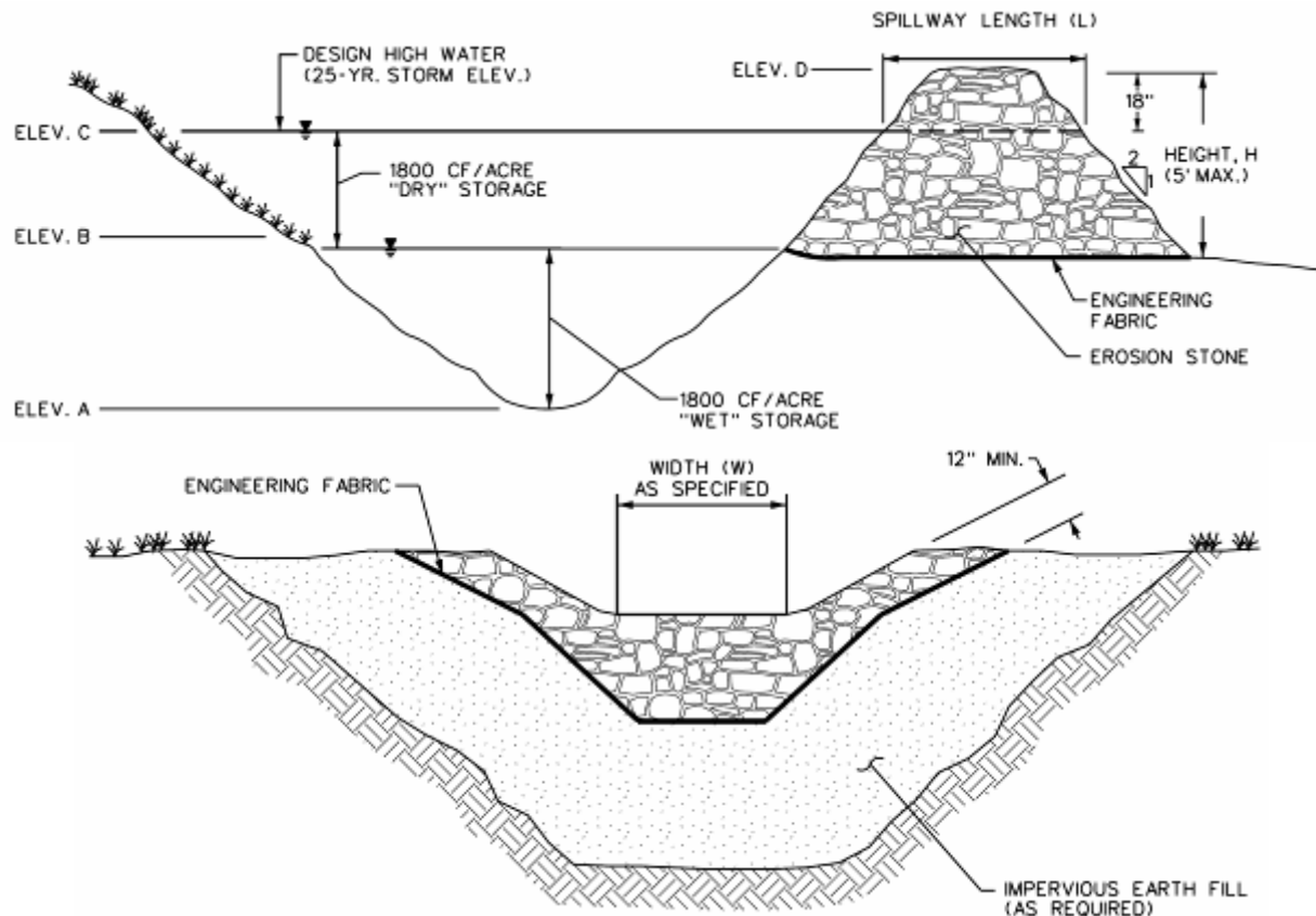
Figure 1: Typical sediment trap with a stone outlet
