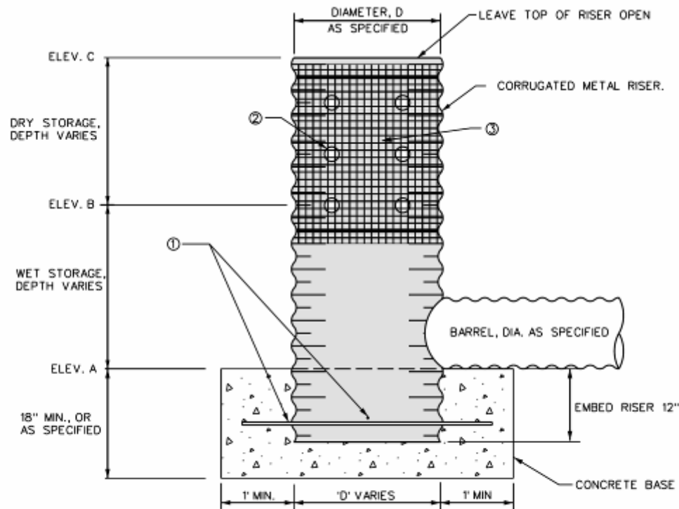
Figure 4: Theoretical discharge orifice for design of perforated risers
