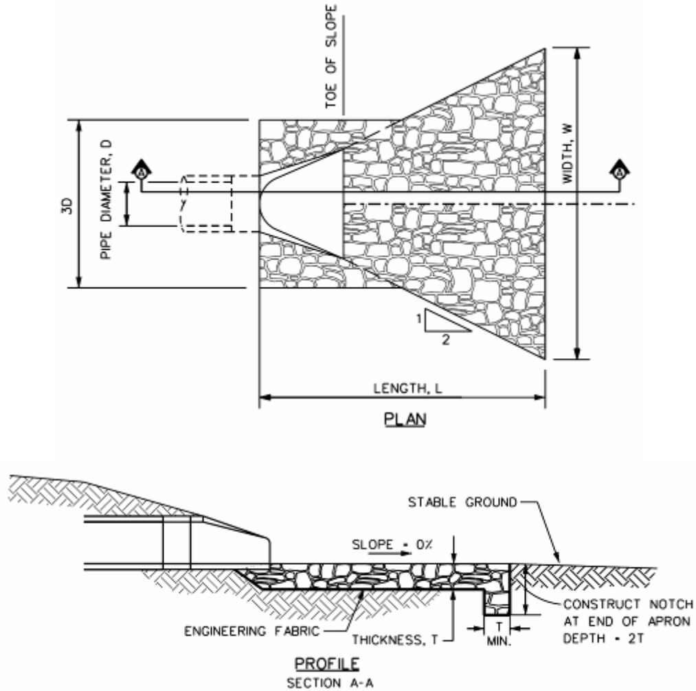
Figure 2: Typical rock apron for outlet to a flat area
