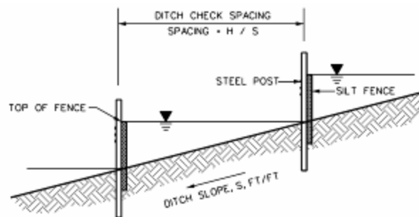
Figure 1: Typical ditch check spacing
