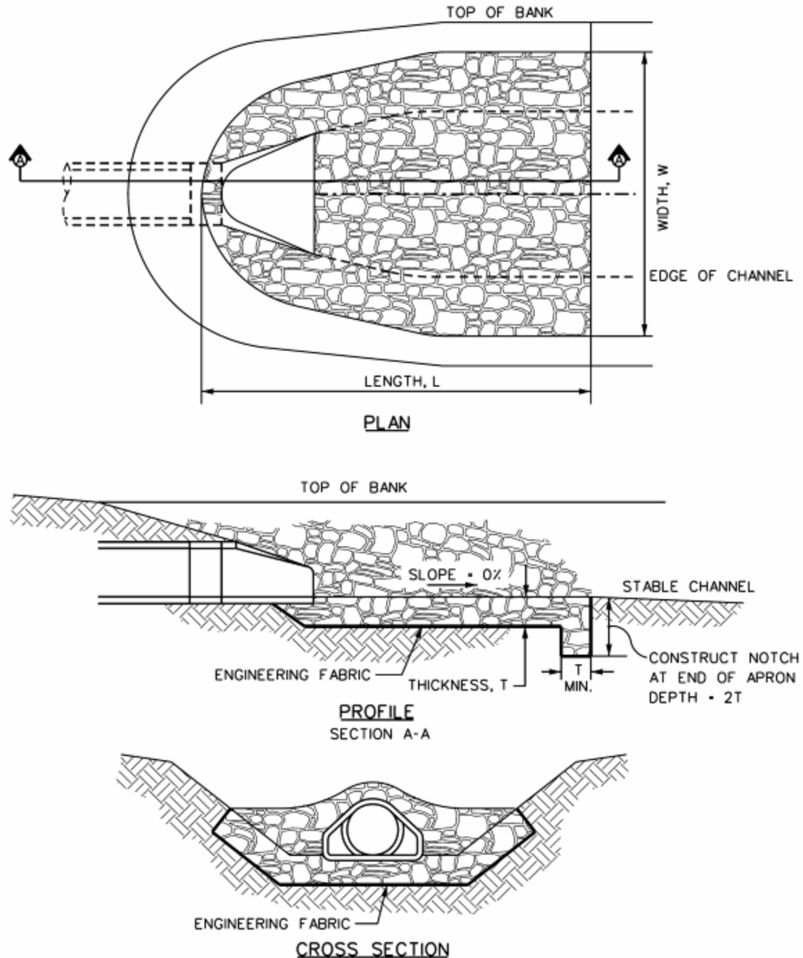
Figure 1: Typical rock apron for outlet to a defined channel
