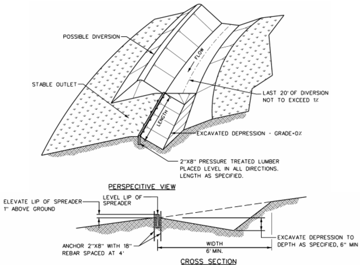
Figure 1: Typical level spreader configuration
