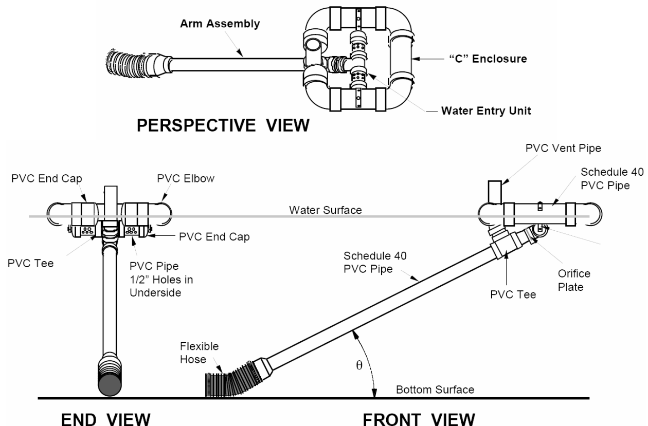
Figure 6: Example skimmer for drawdown of wet storage
