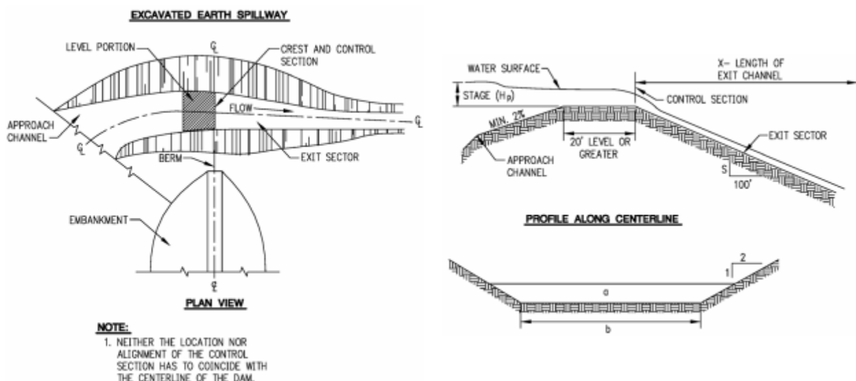
Figure 7: Typical sediment basin emergency spillway
