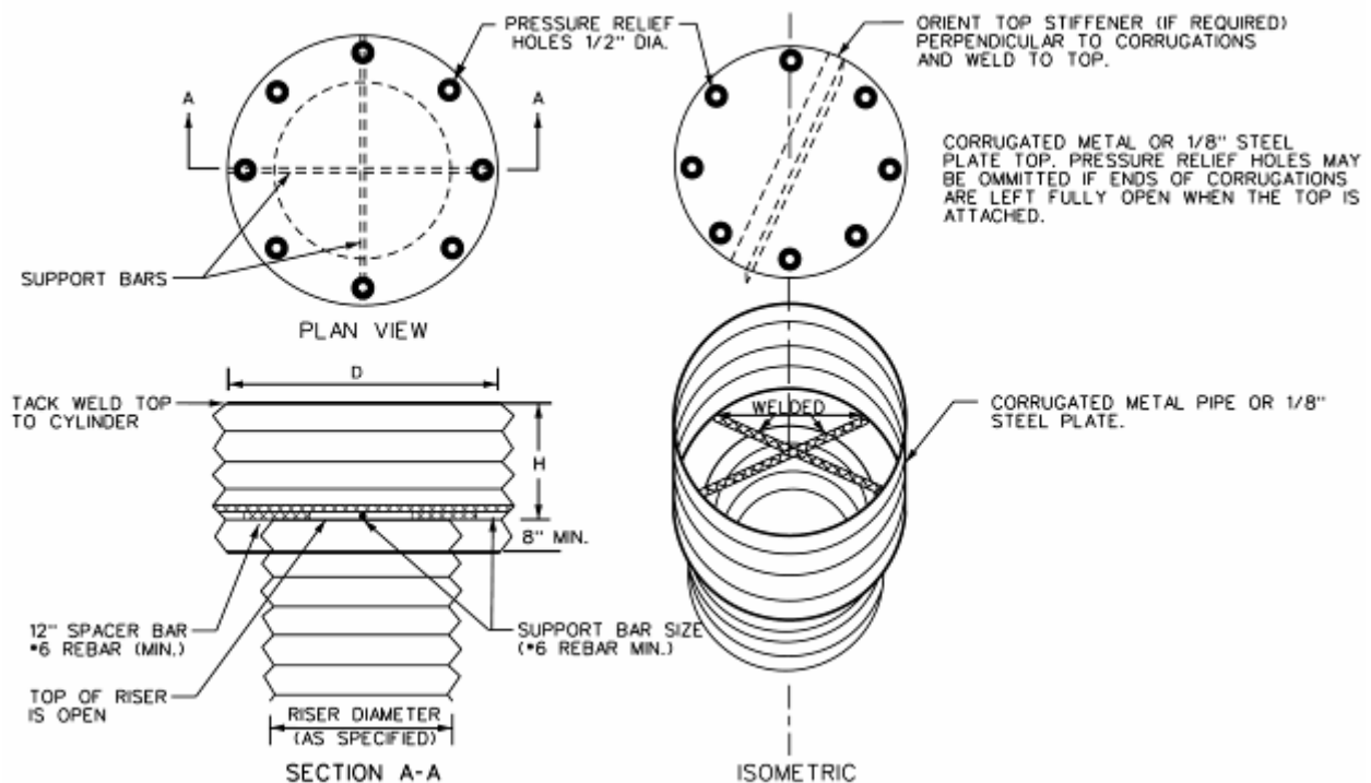
Figure 2: Example anti-vortex device
