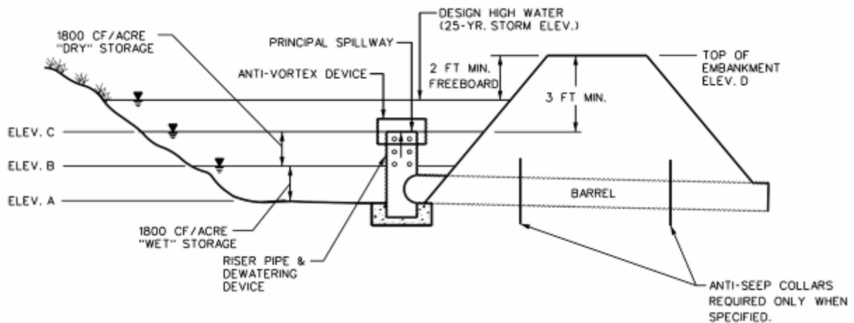
Sediment basin without an emergency spillway
