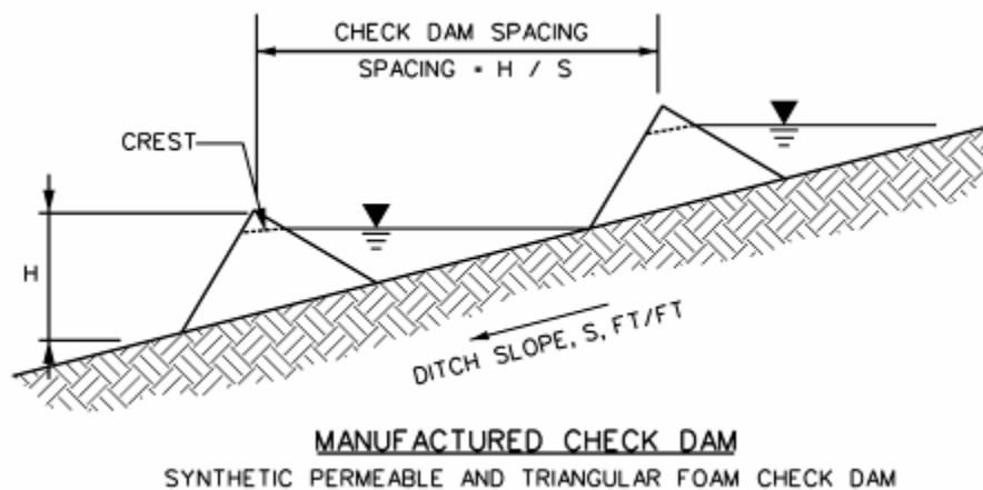
Figure 2: Typical check dam spacing
