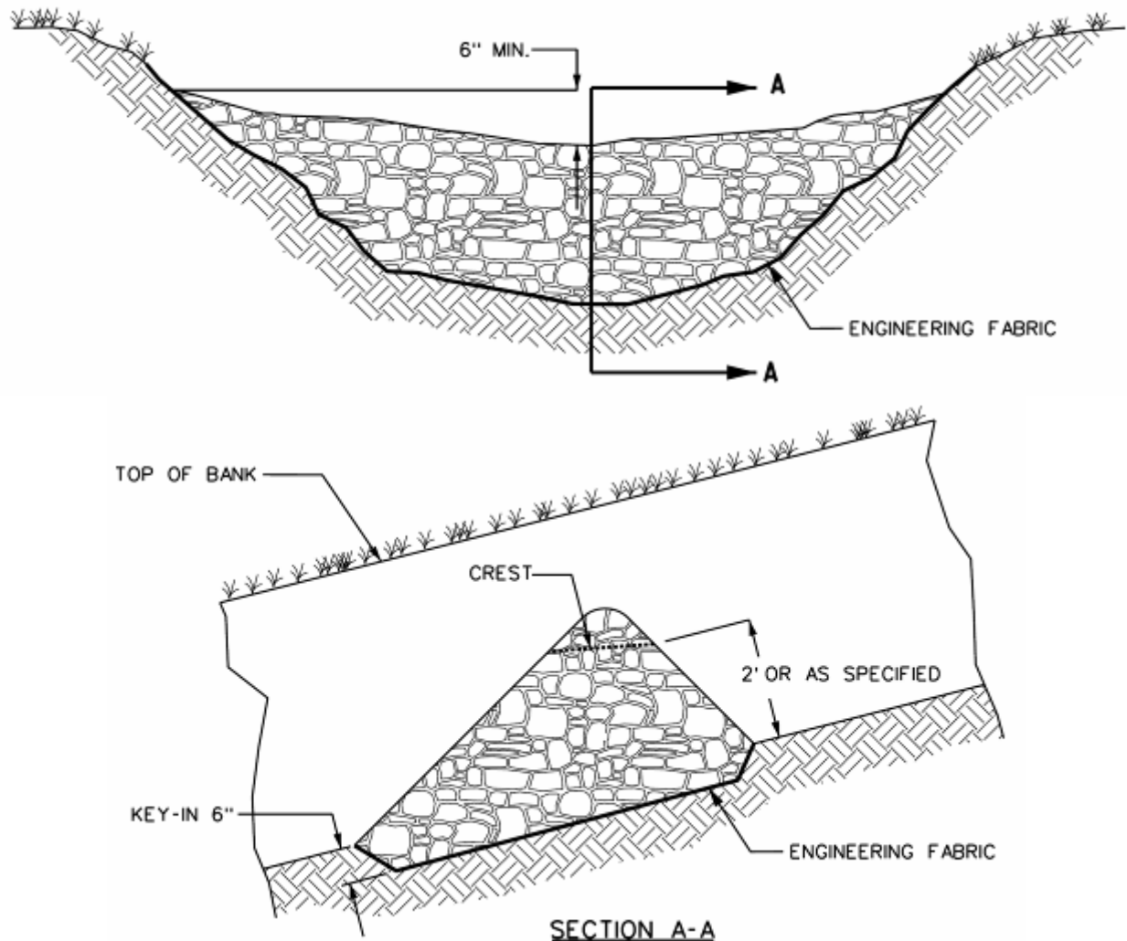
Figure 1: Typical stone check dam
