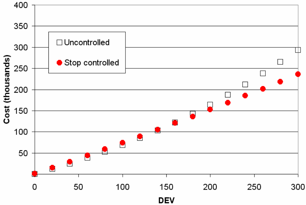
Figure 9. Total cost in ten years based on control type
