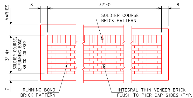
PIER CAP SIDE DETAIL
