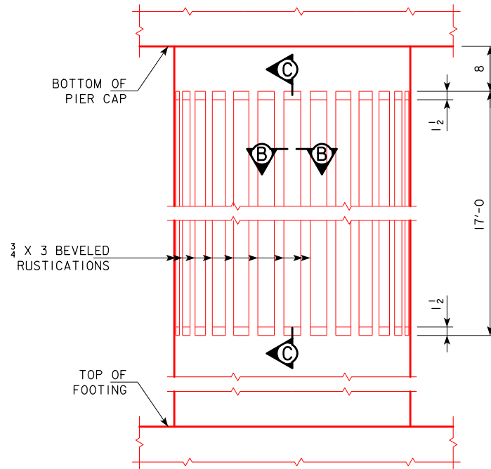
COLUMN DETAIL
