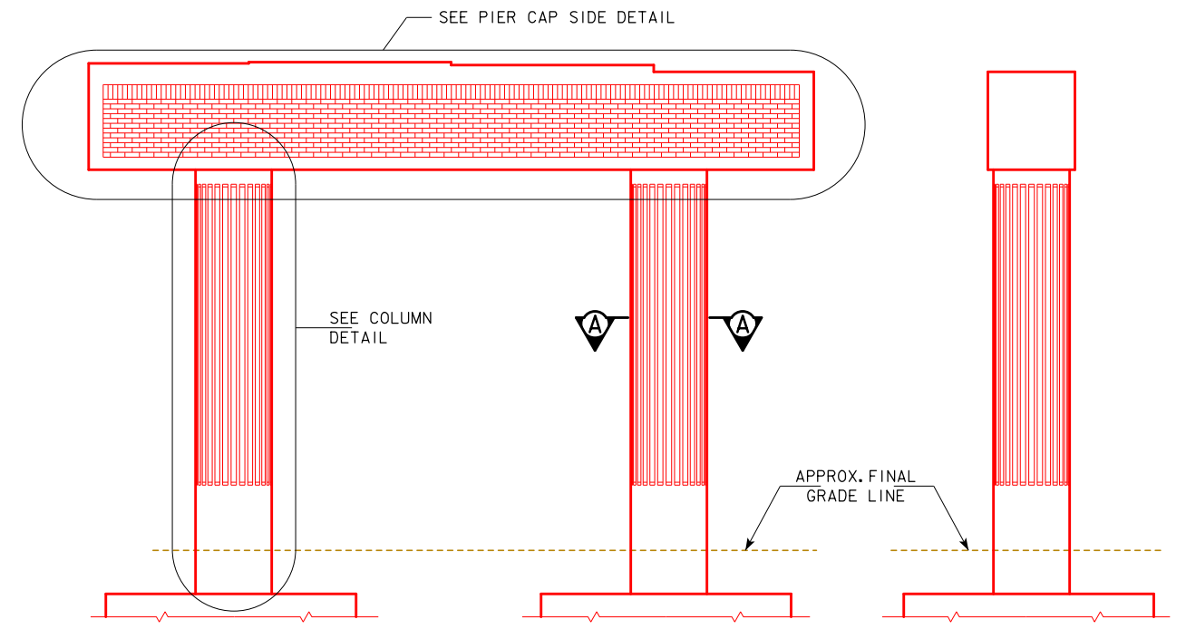
PIER SIDE ELEVATION
