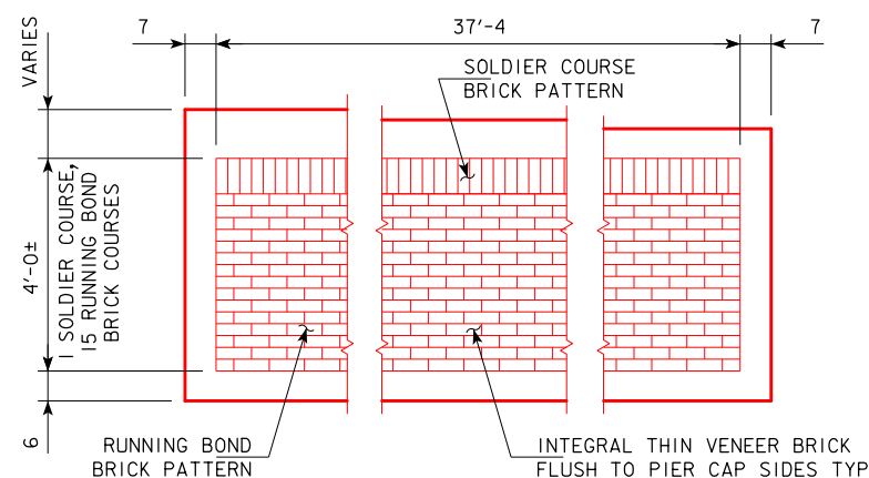
PIER CAP SIDE DETAIL
