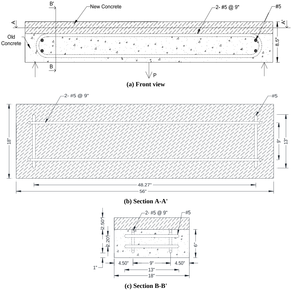
Figure 41. Positive bending flexural test specimen schematic (Case 1)
