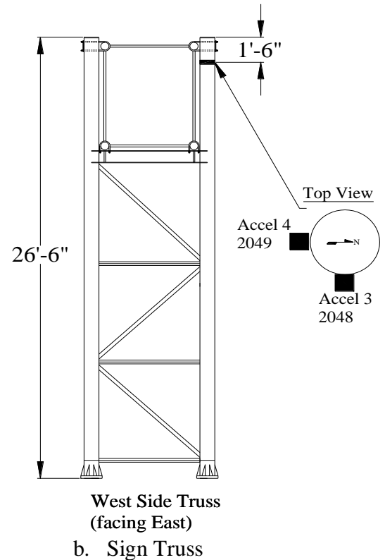
Fig. 47 Ankeny DMS/Sign Truss instrumentation configuration at Cross Section B.
