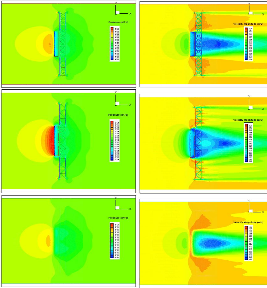
Fig. 13 Distribution of pressure (left) and velocity magnitude (right) in three horizontal planes cutting under the DMS (top), through the DMS (middle) and over the DMS (bottom) in the simulation (Case B) in which the DMS cabinet is attached to the truss. The wind speed is 90 mph. Wind direction is from left to right.
