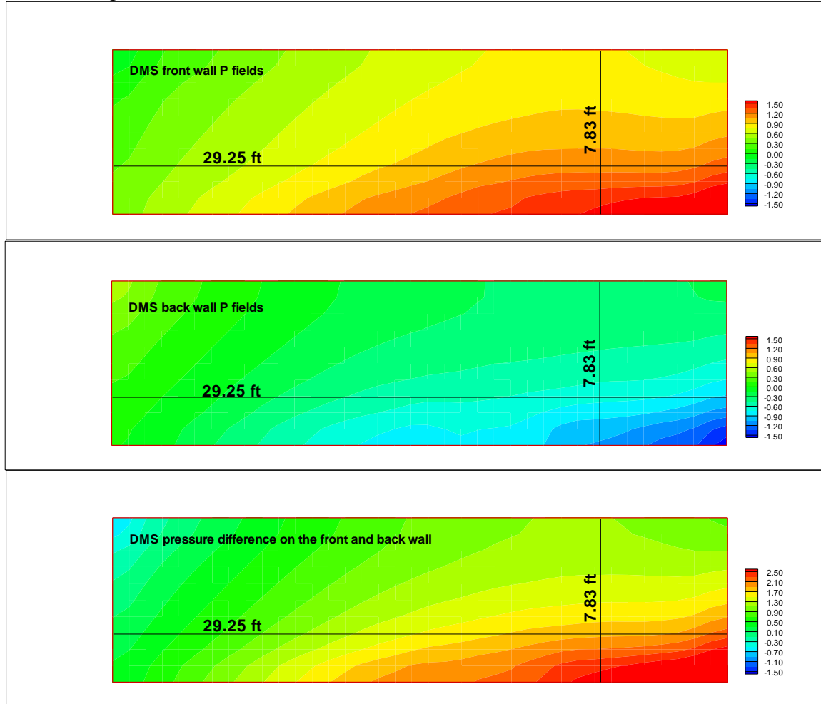
Fig. 18 Non-dimensional pressure distributions, p/\rho U^2 \cdot 1000 , on the front and back faces of the DMS cabinet for the case of a ‘very long’ truck and no wind. Last frame shows the distribution of the non-dimensional pressure difference between the two faces, \Delta p/\rho U^2 \cdot 1000 .
