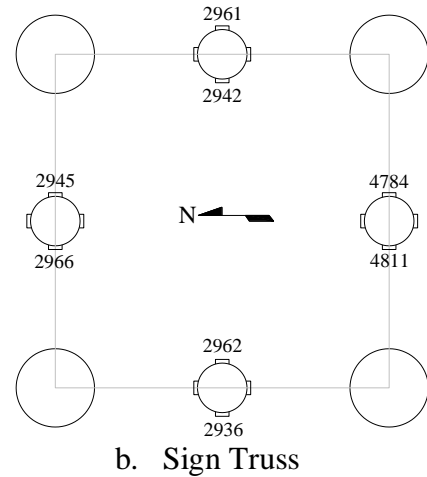
Fig. 47 Ankeny DMS/Sign Truss instrumentation configuration at Cross Section B.
