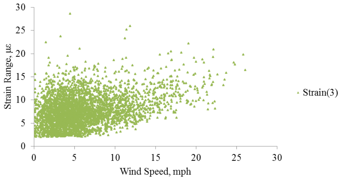
c) Strain range 3 in chord member gages
