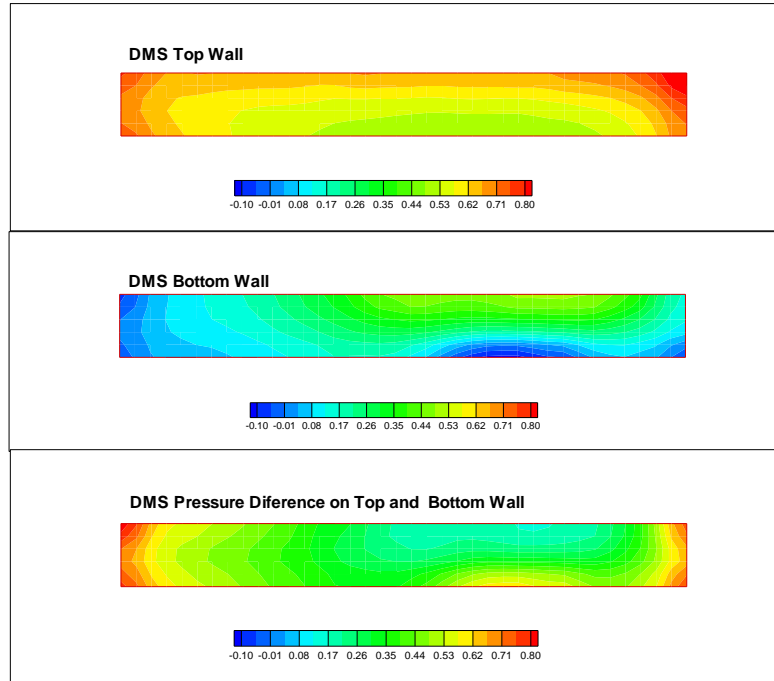
Fig. 19 Non-dimensional pressure distributions, p/\rho U^2 \cdot 1000 , on the bottom and top faces of the DMS cabinet for the case of a ‘very long’ truck and no wind. Last frame shows the distribution of the non-dimensional pressure difference between the two faces, \Delta p/\rho U^2 \cdot 1000 .
