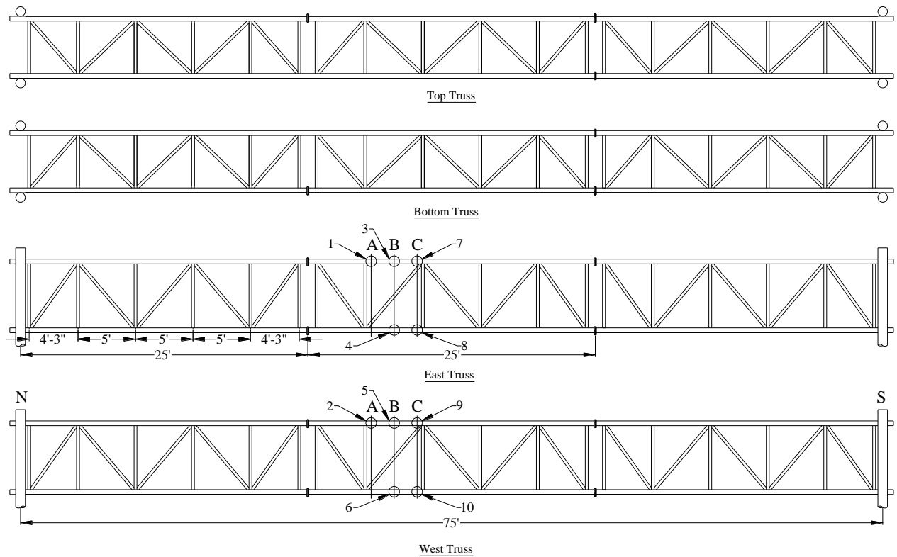
Fig. 35. Truss configuration and gage locations for Kellogg DMS truss
