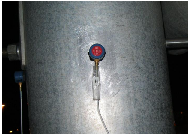
Fig. 29 View of an accelerometer attached to a truss member
