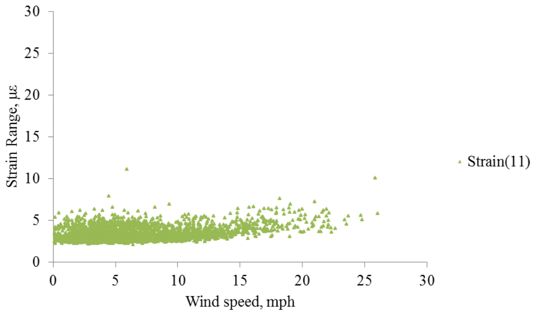
k) Strain range 11 in chord member gages
