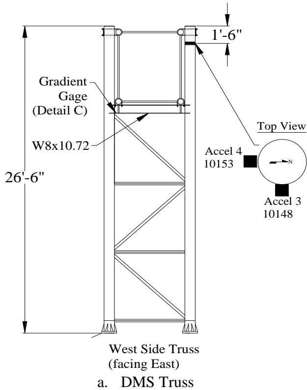
Fig. 47 Ankeny DMS/Sign Truss instrumentation configuration at Cross Section B.
