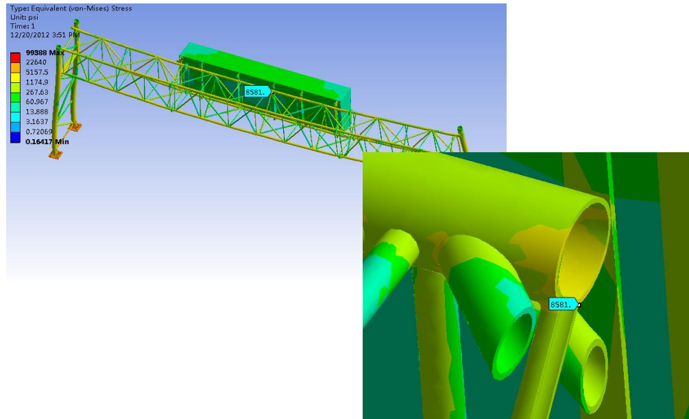
Fig. 84 Maximum stress on diagonal welding
