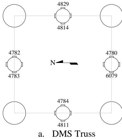
Fig. 47 Ankeny DMS/Sign Truss instrumentation configuration at Cross Section B.
