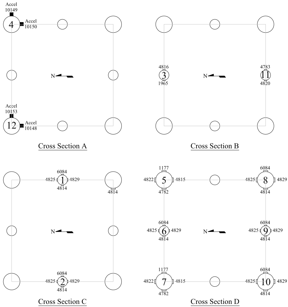
Fig. 40 Euclid (I235) DMS Truss chord and diagonal instrumentation configuration.
