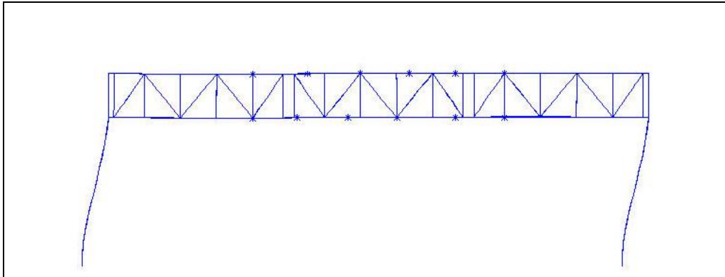
Fig. 22 Truss deformations for the case where DMS cabinet was modeled as point mass units that where evenly distributed where the DMS cabinet attaches to the truss, first frequency
