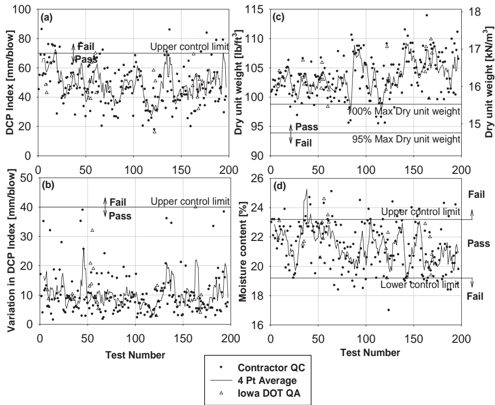
Control charts for unsuitable soil D
