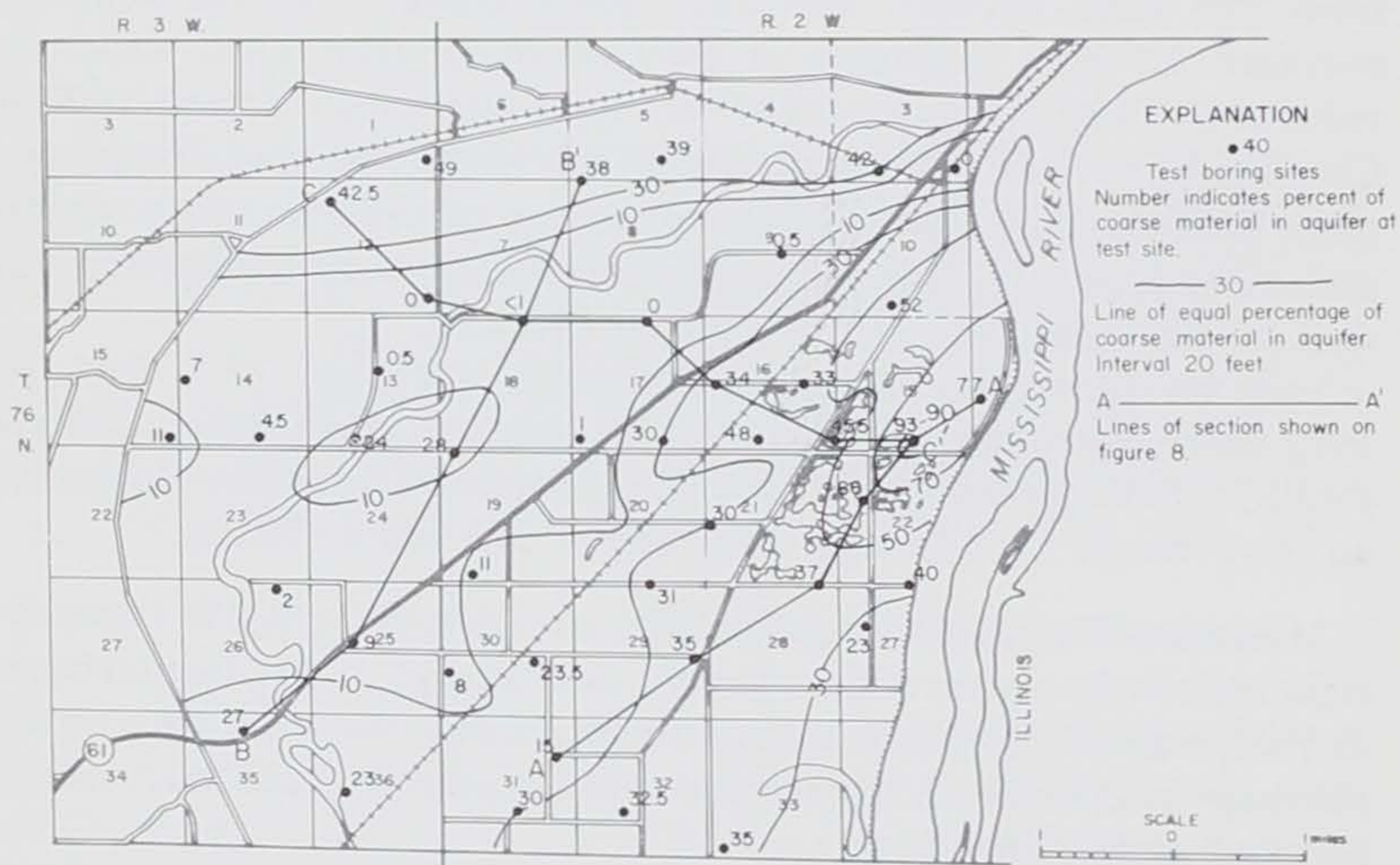
Figure 7.—Percent of coarse material in the aquifer.
