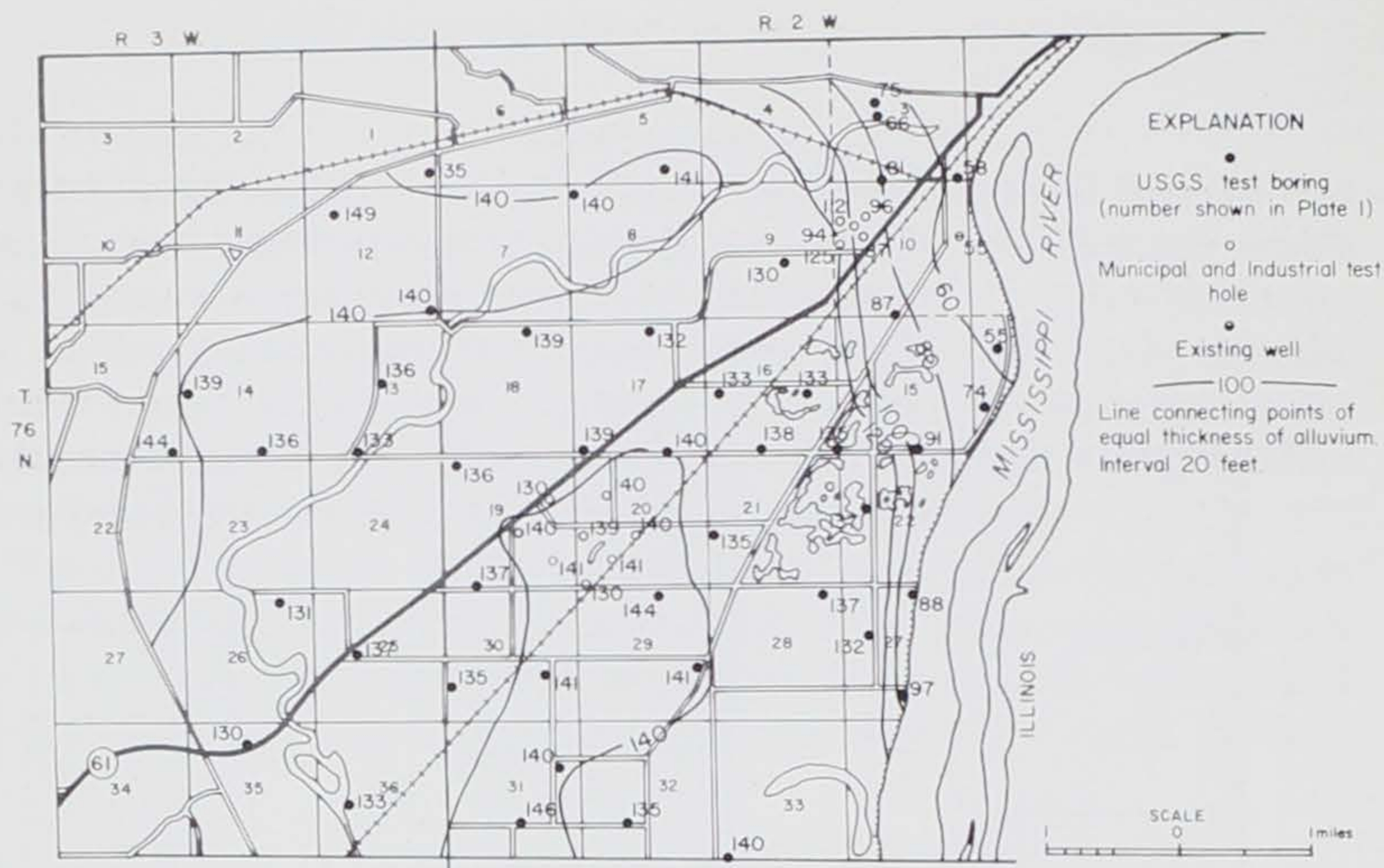
Figure 9.—Thickness of alluvium.
