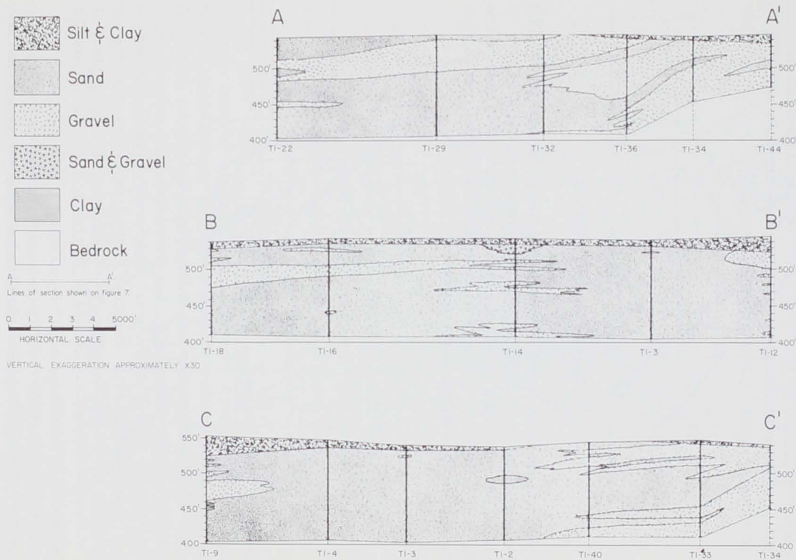
Figure 8.—Geologic sections of the aquifer.
