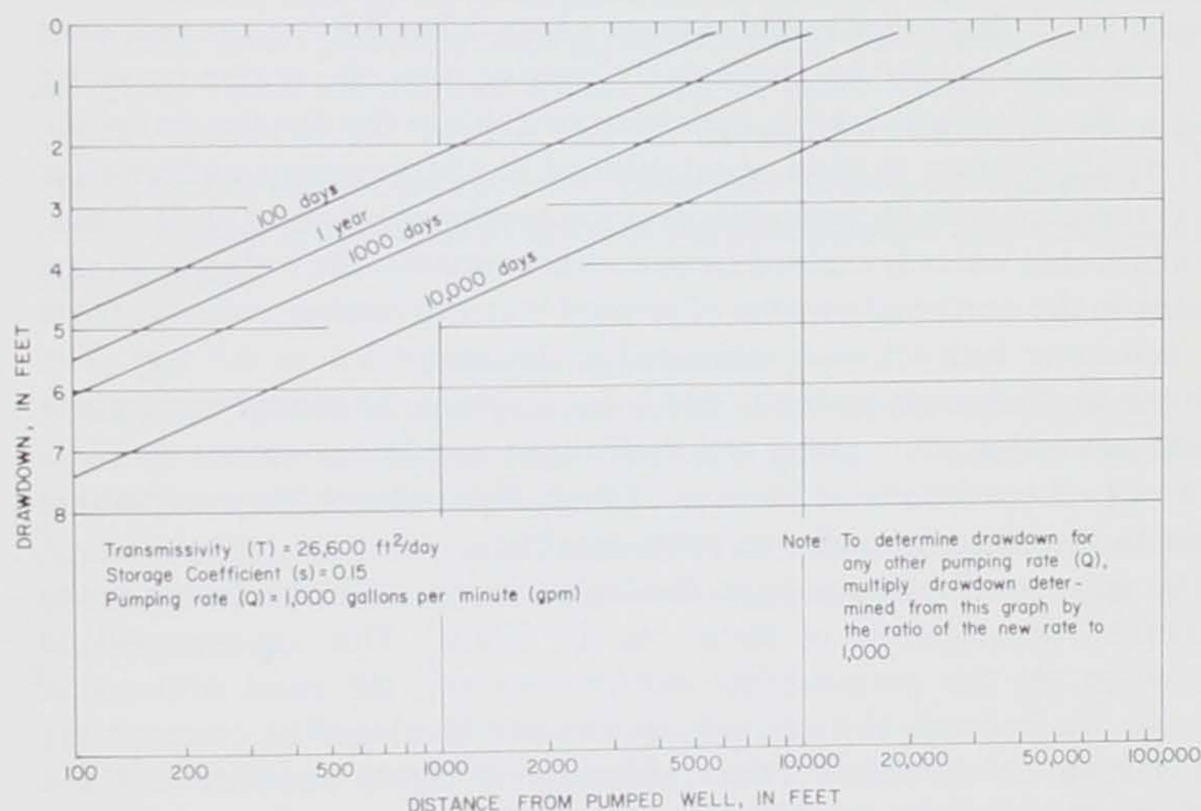
Figure 28.—Distance-drawdown graph.
