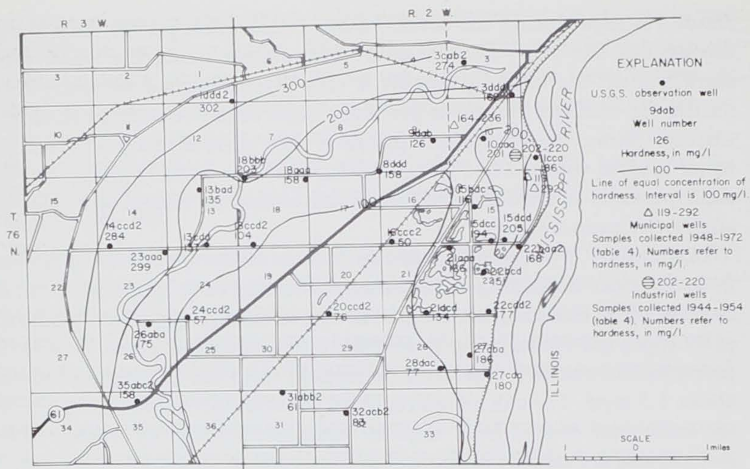
Figure 20.—Distribution of hardness in water from shallow wells in the alluvial aquifer.
