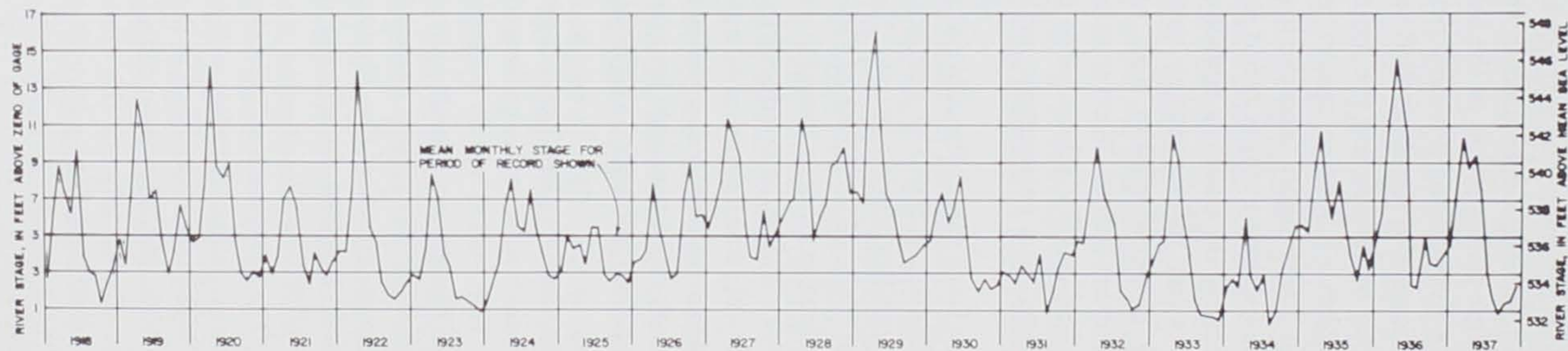
Figure 16.—Monthly mean stage of Mississippi River at Muscatine gage—1918 through 1937.
