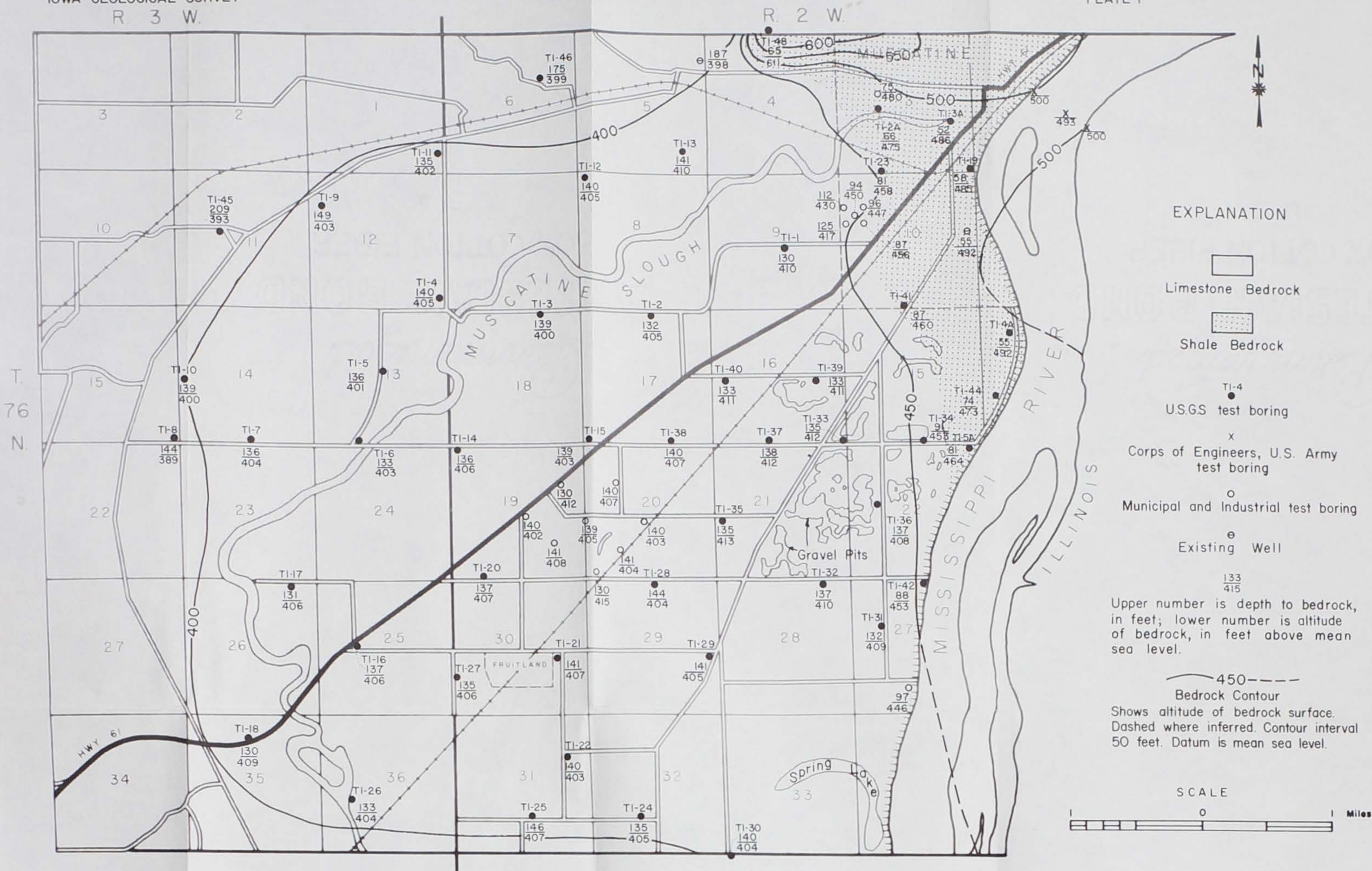
THE BEDROCK SURFACE - ITS ALTITUDE, CONFIGURATION, AND LITHOLOGY.
