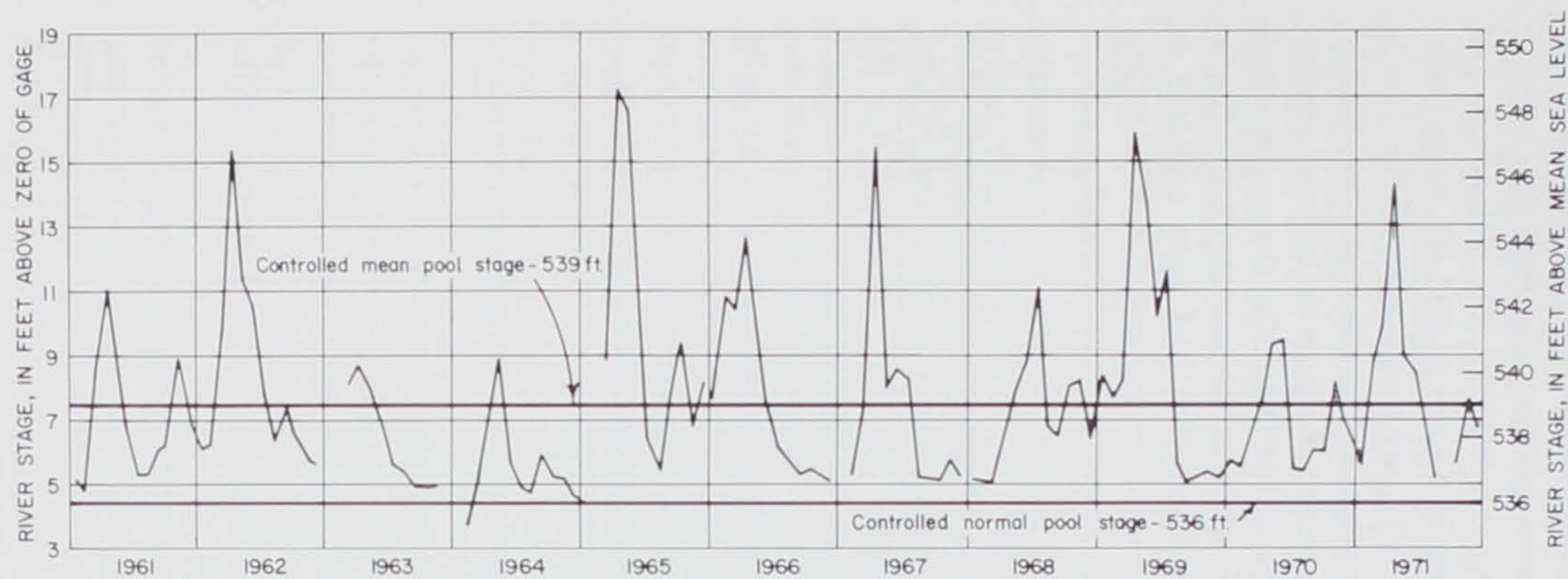
Figure 15.—Monthly mean stage of Mississippi River at Muscatine gage—1961 through 1971.
