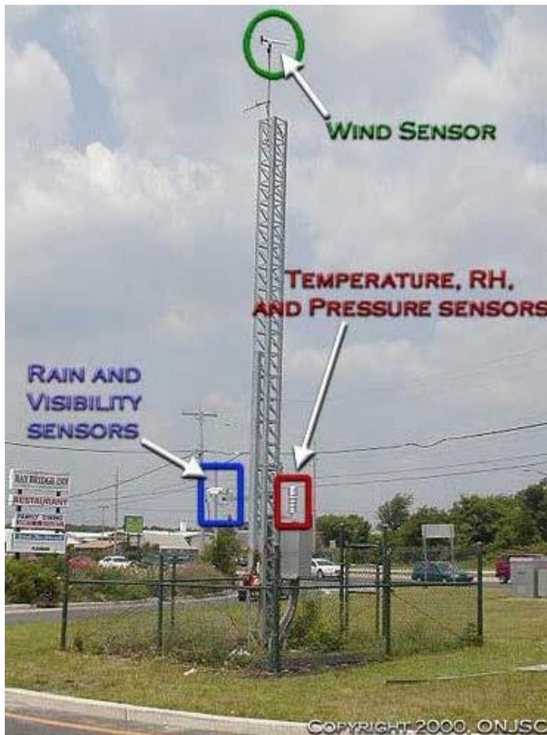
Figure 4. Example of an RWIS sensor station (Copyright 2000 Office of the New Jersey State Climatologist (ONJSC))
