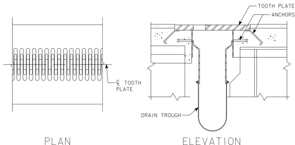
Figure 1.1-2. Finger Joint
