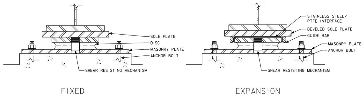
Figure 5.1-4. Disc Bearings
